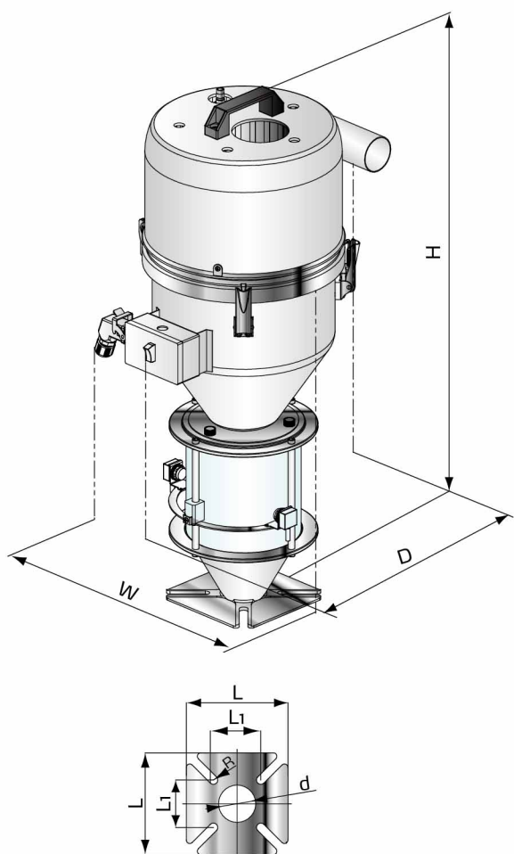
SHR-U-EST底座安裝尺寸
