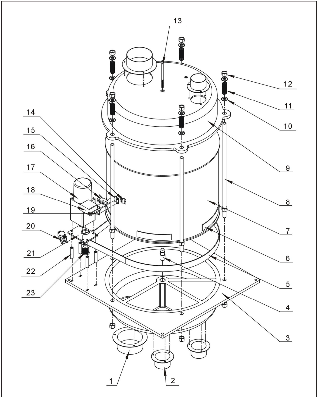
Picture 2-7: Optional Honeycomb (dew-point: -50^{\circ}\text{C} ) Parts Drawing (SCD-900U/700H 1200U/700H)
